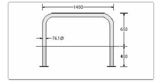
Marshalls Rino Steel Hoop barrier RB76 Black in colour
